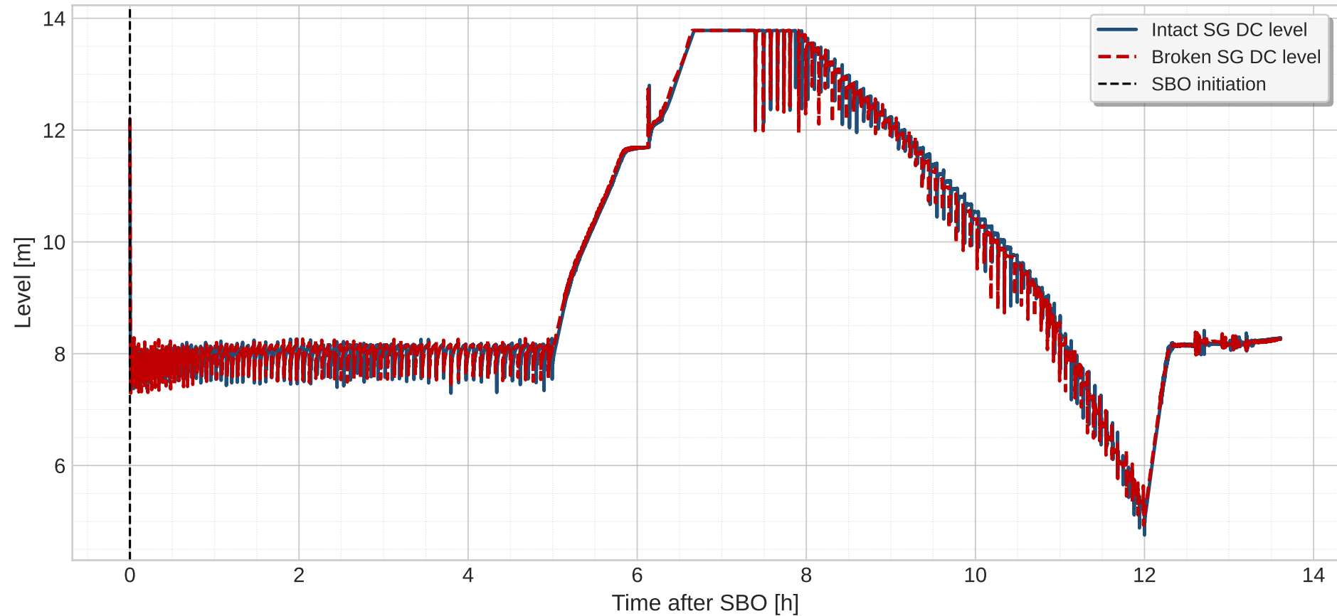
No SG Depressurization - Steam Generator DC Levels
